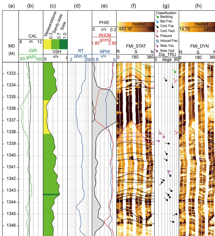
Fig. 9 Key geophysical logs and the FMI image of the 1334–1346 m MD fault core. The geophysical logs denote the lithology (GR and Vsh logs) and porosity (PHIE, RHOB, NPHI, and RT logs). The two most fractured intervals within the fault core are 1334–1339 and 1343–1346 m MD. The 1334–1339 m interval developed in the metasandstones (low GR) with extremely high porosity (low RT, low RHOB, and high NPHI values). This interval is the most permeable interval in the studied well section. The attitude of the bounding fault planes at 1334 and 1338 m MD is about N50E/75–80°NW
